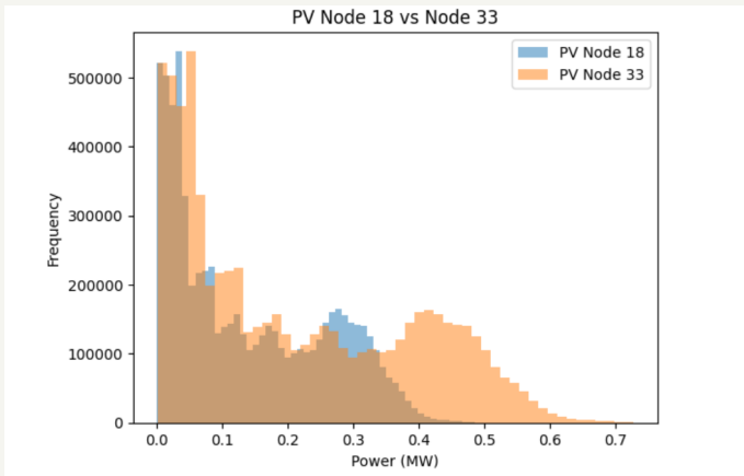
Fig : This histogram compares the power output distribution of PV Node 18 and 33.
