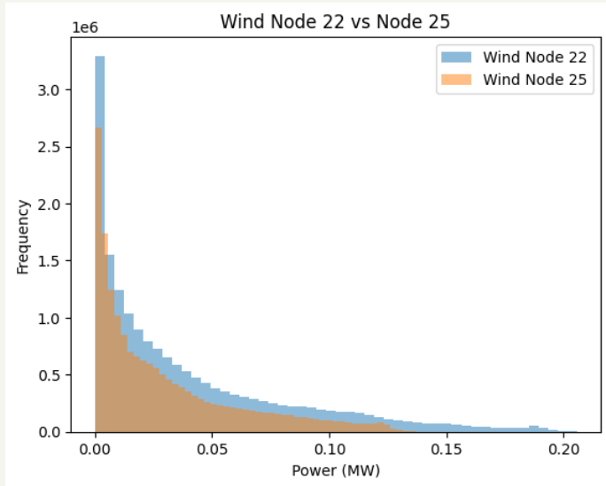
Fig : This histogram compares the power output distribution of Wind Node 22 and 25.
